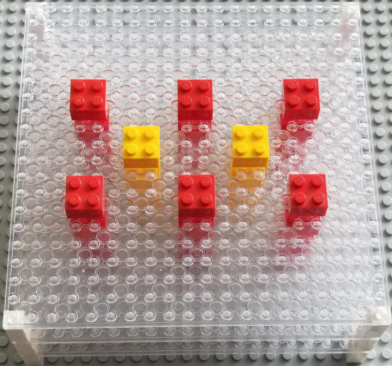
A crystal example - top view
