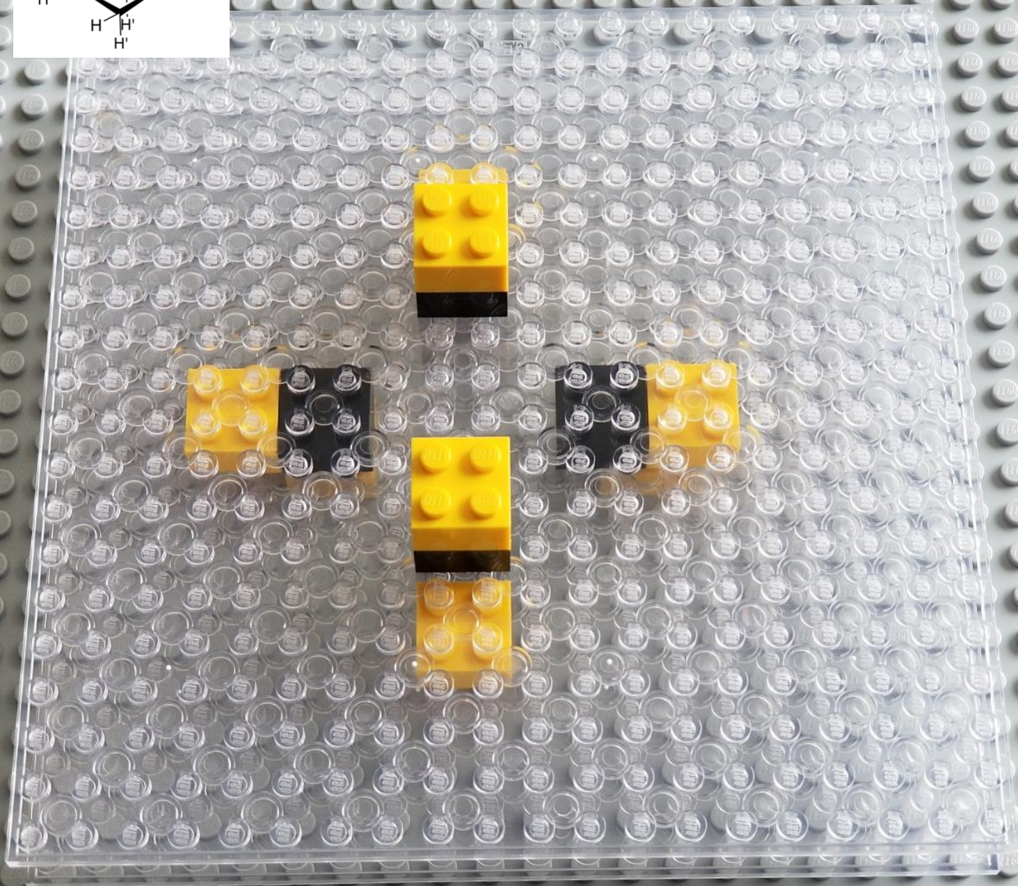
A cyclobutane conformation – top view
